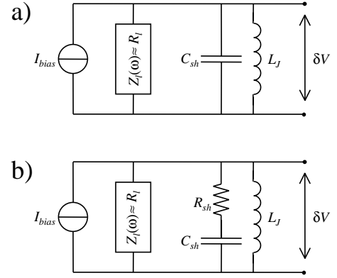
Fig. 4. Circuit models for the C -shunted DC-SQUID (a) and the RC -shunted DC-SQUID (b). The SQUID is modeled as an inductance L_J . A shunt circuit, the superconducting capacitor C_{sh} or the R_{sh} - C_{sh} series, is fabricated on chip very close to the SQUID. The noise that couples to the qubit results from Johnson-Nyquist voltage noise \delta V from the circuit's total impedance Z_t . Z_t is formed by a parallel combination of the impedances of the leads Z_l , the shunt and the SQUID, such that Z_t = (1/Z_l + 1/(R_{sh} + 1/i\omega C_{sh}) + 1/i\omega L_J)^{-1} , with R_{sh} = 0 for (a).
