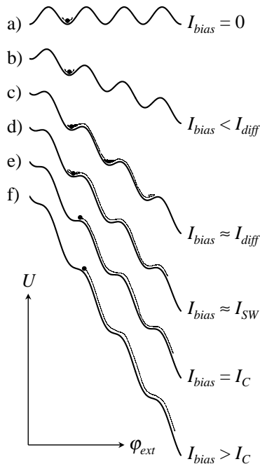
Fig. 3. The dynamics of a current-biased DC-SQUID, modeled as a particle with coordinate \varphi_{ext} in a one-dimensional tilted washboard potential U . The labeling (a)–(f) corresponds to that of Figure 2. At zero (a) and small bias currents (b), the particle is trapped in a well of the washboard. Apart from the small plasma oscillations at the bottom of the well, the particle’s coordinate \varphi_{ext} is fixed. When increasing the slope of the washboard, the particle will start to have a slow, on average downwards, diffusive dynamics, with rare excursions to one of the neighboring wells (c). At the switching current I_{SW} there is a high probability that the trapped particle will escape to a running mode (d), with effectively zero probability for retrapping. Here the loss of potential energy exceeds the dissipation when the particle moves one period down the washboard, and the particle builds up a high kinetic energy. Due to thermal fluctuations, external noise, and in certain cases quantum fluctuations, this occurs below the critical current I_C : the slope where all local minimums in the washboard potential disappear (e). At currents higher than this slope (f), the particle will always be in a running mode. The retrapping process when lowering the bias current follows similar dynamics.
