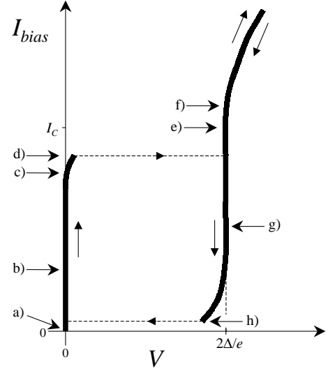
Fig. 2. Sketch of a typical hysteretic current-voltage characteristic ( IV ) for a current-biased Josephson junction or small DC-SQUID. The IV is hysteretic; arrows indicate which of the two branches is followed at an increase or decrease of the bias current. When the bias current I_{bias} is ramped up from zero (a), the voltage V first remains zero. The circuit is here on the supercurrent branch of the IV (b). When I_{bias} approaches the critical current I_C , a slow diffusive motion of the phase \varphi_{ext} leads to a very small voltage across the system (c). At slightly higher current (d), but always below I_C (e), the system switches to a running mode for \varphi_{ext} , and the voltage jumps to a value set by quasiparticle tunneling over the superconducting gap, V = 2\Delta/e (this current level (d) is the switching current I_{SW} ). At further increase of the current (f) the IV approaches an Ohmic branch, where transport is dominated by quasiparticle tunneling through the normal tunnel resistance of the junctions. When lowering the bias current the system follows the running mode (g) down to a low bias current where it retraps on the supercurrent branch (at the level I_{retrap} , indicated by (h)). See also the corresponding washboard potential model, in Figure 3.
